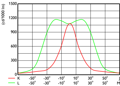
OFCS1_BVP140T251xLED480-4S740S
