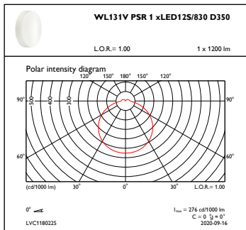
OFPC1_WL131VPSR1xLED12S830D350
