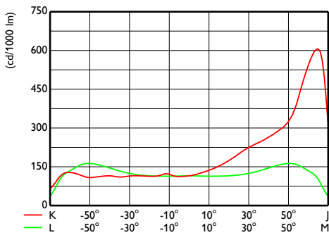
OFCS1_BVP650T251xLED340-4S740DX50
