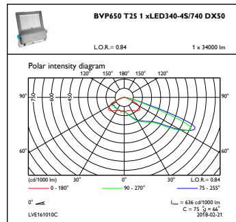
OFPC1_BVP650T251xLED340-4S740DX50
